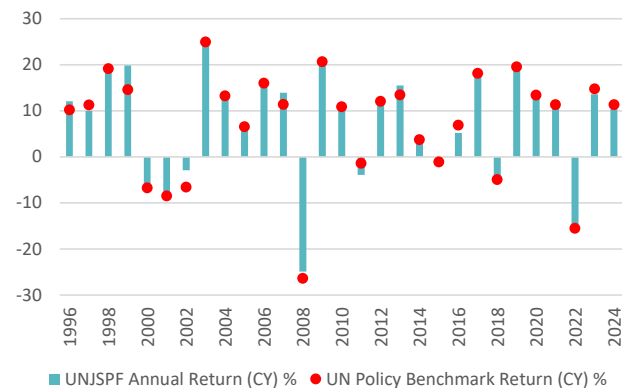
Annual Return Calendar Year (%)
